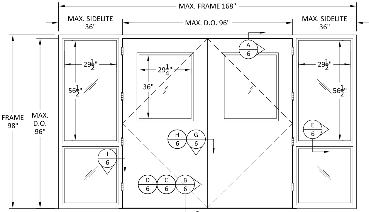
ELEVATION OXXO (OUTSWING DOOR - EXTERIOR VIEW)
