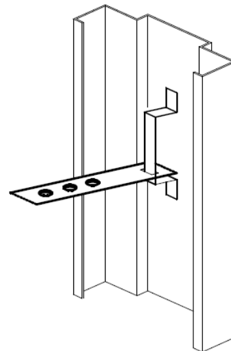
D 7 ISOMETRIC JAMB MASONRY - 14 GA. YOKE & STRAP
