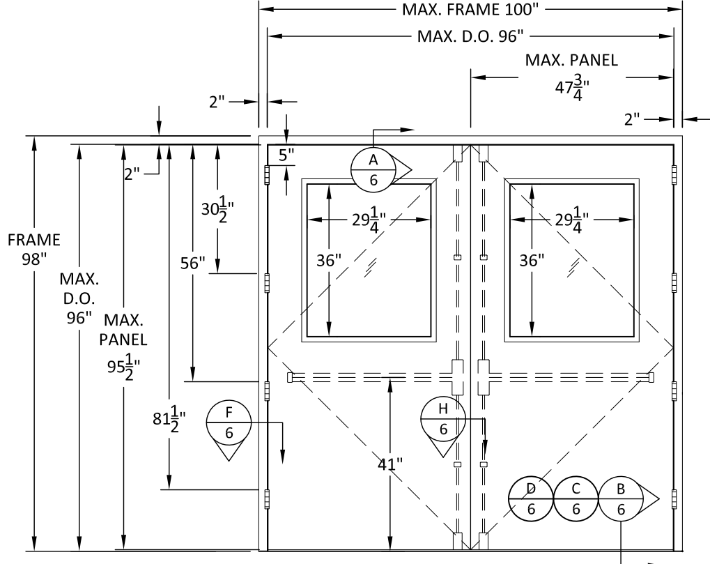
ELEVATION PAIR SARGEANT HC8713 SURFACE VERTICAL ROD EXIT DEVICE (OUTSWING DOOR - EXTERIOR VIEW)
