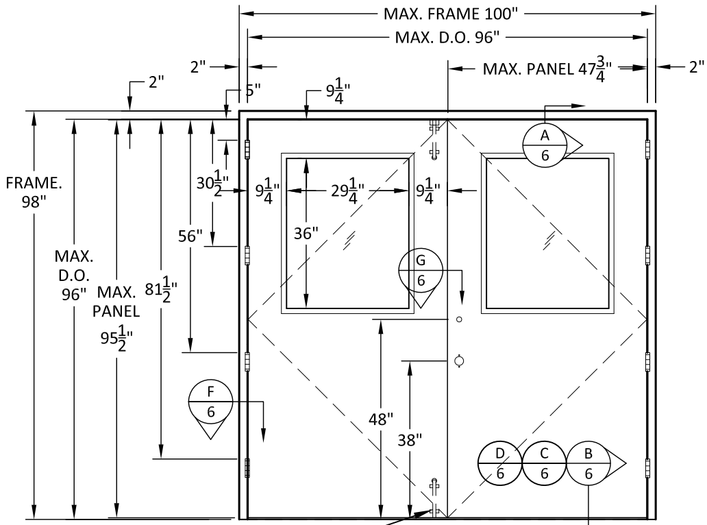
ELEVATION PAIR SURFACE BOLTS YALE SECURITY SURFACE BOLT KIT 988 OR ROCKWOOD 556 WS FLUSH BOLT X 12" KIT CORBIN RUSSWIN CL3300 CYL. LOCK WITH DEADLOCK DL4113 (OUTSWING DOOR - EXTERIOR VIEW)
