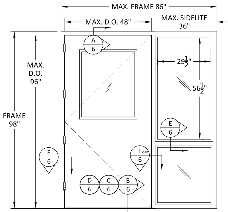
ELEVATION XO, OX (OUTSWING DOOR - EXTERIOR VIEW)
