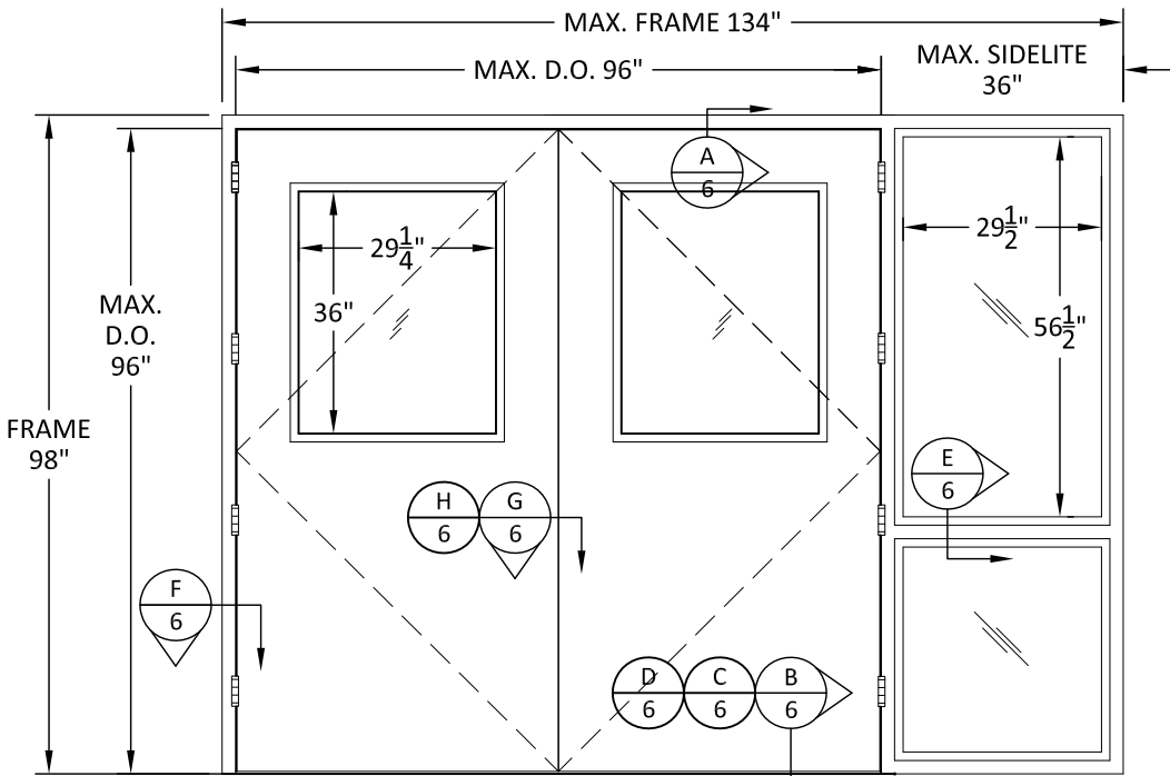
ELEVATION XXO, OXX (OUTSWING DOOR - EXTERIOR VIEW)
