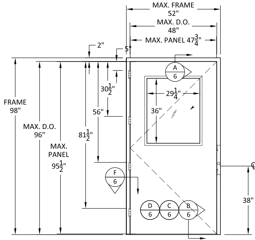
ELEVATION SINGLE SS10300 JAMB MOUNTED LOCK (OUTSWING DOOR - EXTERIOR VIEW) MAY ALSO UTILIZE CYLINDRICAL LOCK WITH DEAD BOLT, MORTISE LOCK, OR SURFACE VERTICAL RODS
