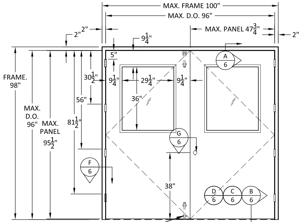
ELEVATION PAIR SURFACE BOLTS YALE SECURITY SURFACE BOLT KIT 988 OR ROCKWOOD 556 WS FLUSH BOLT X 12" KIT SCHLAGE L9080P MORTISE LOCK (OUTSWING DOOR - EXTERIOR VIEW)
